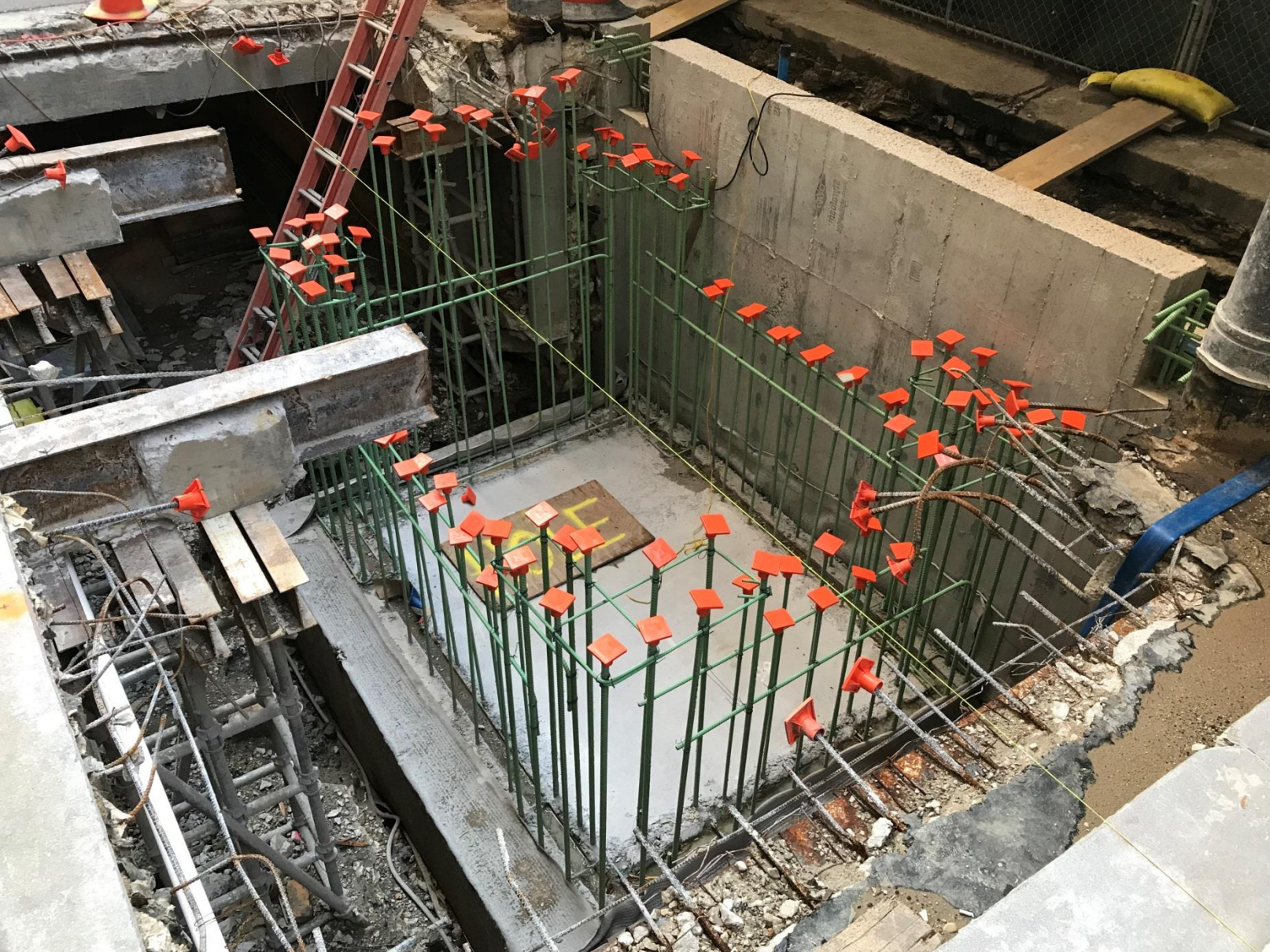
East Elevator Foundation Wall Build Out
