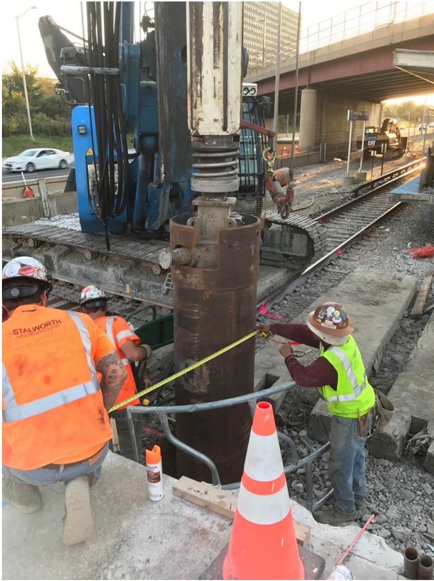
Ogden Stationhouse – Caisson Installations
