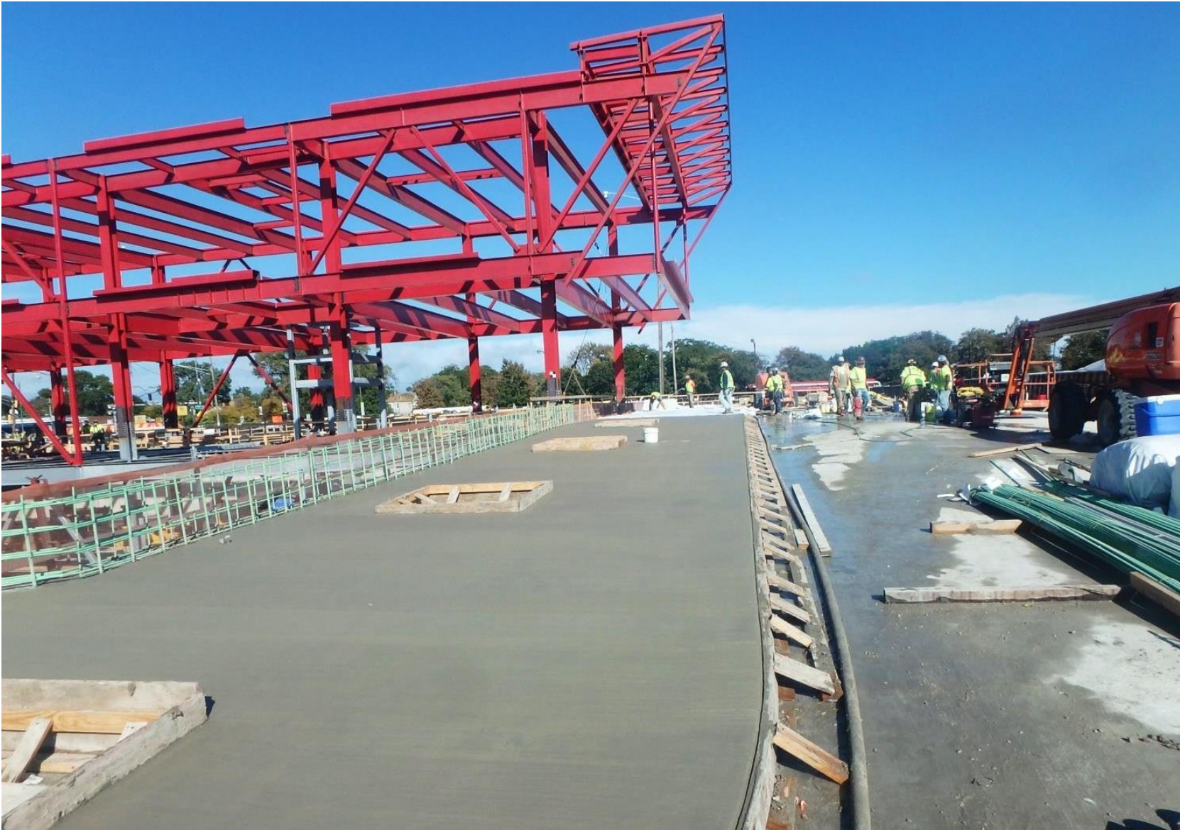
South Bus Bridge - Sidewalk Poured
