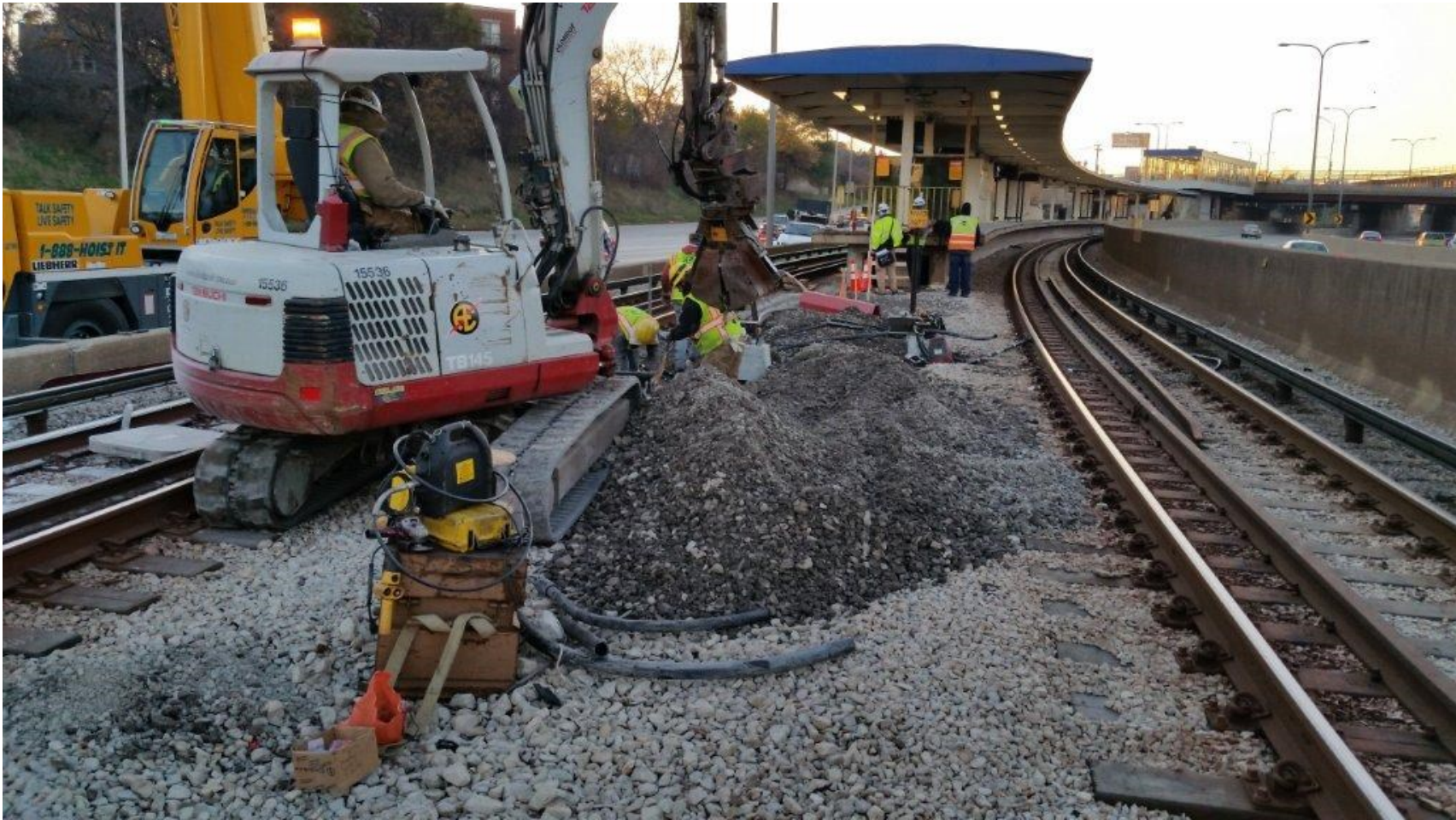
Addison Relocation of Signal Equipment
