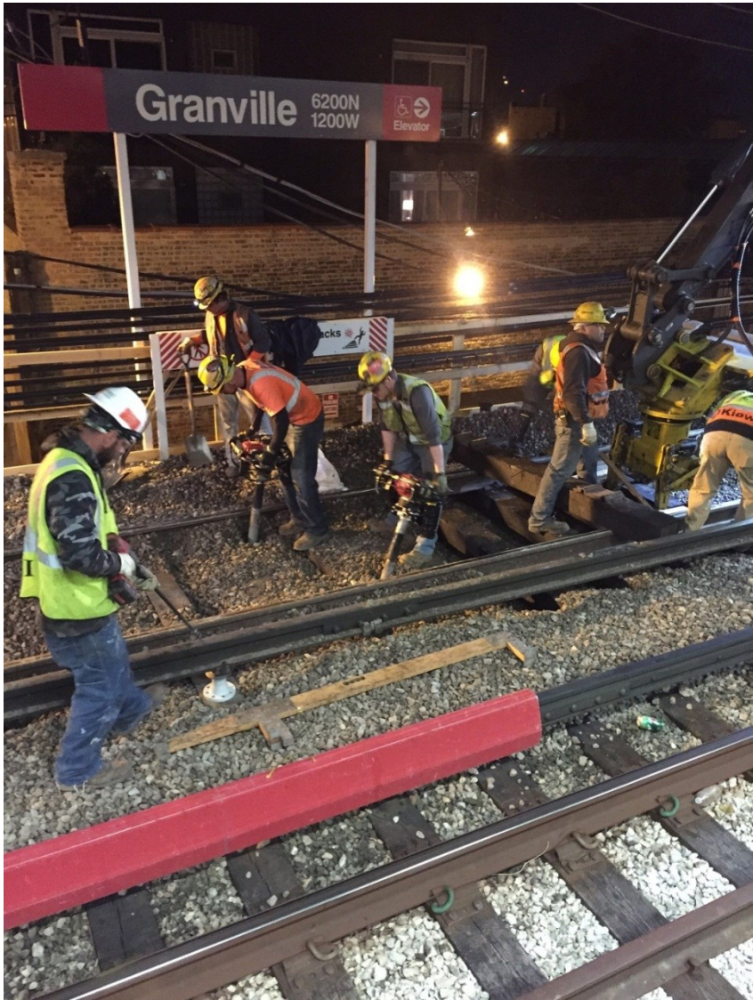
Kiewit crews performing tie replacement.
