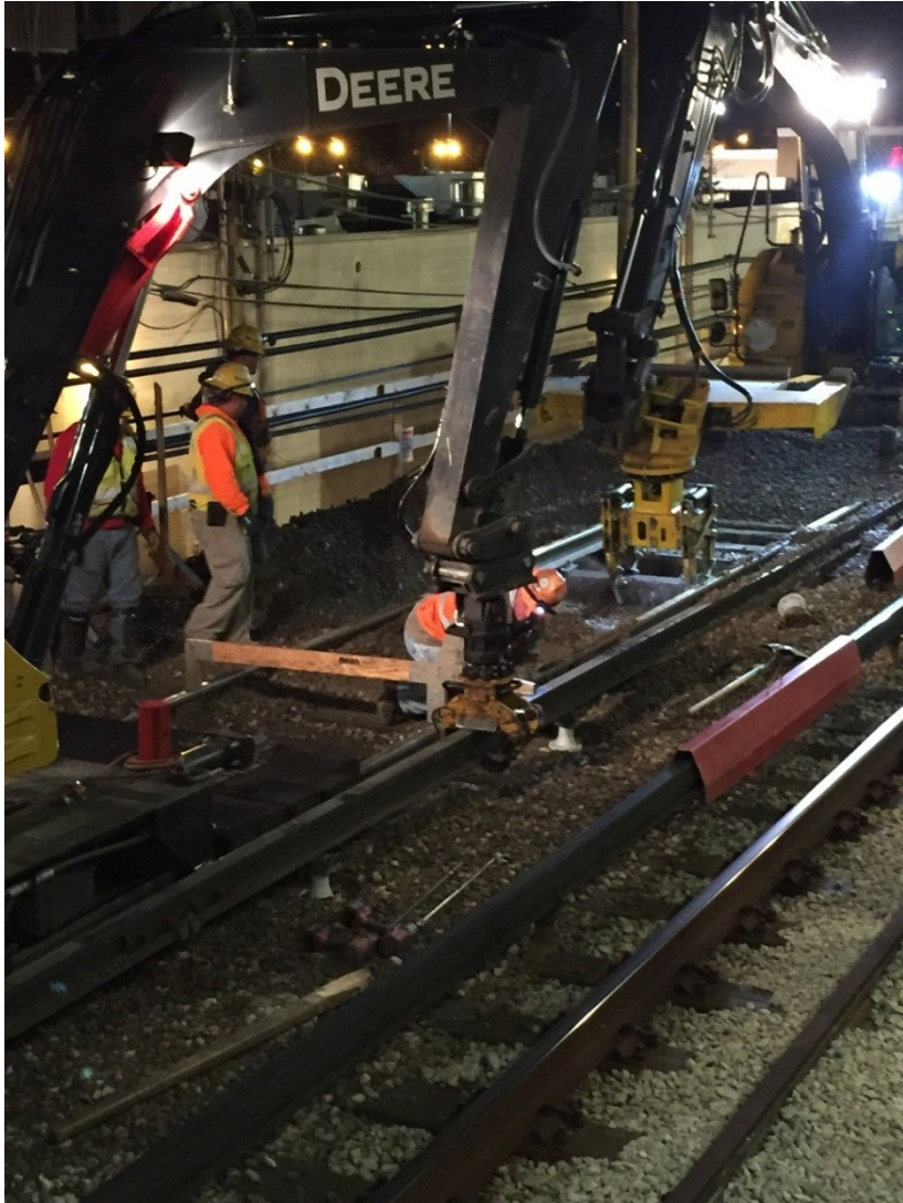
Track 1 replacement, gauging and alignment, ballast restoration.
