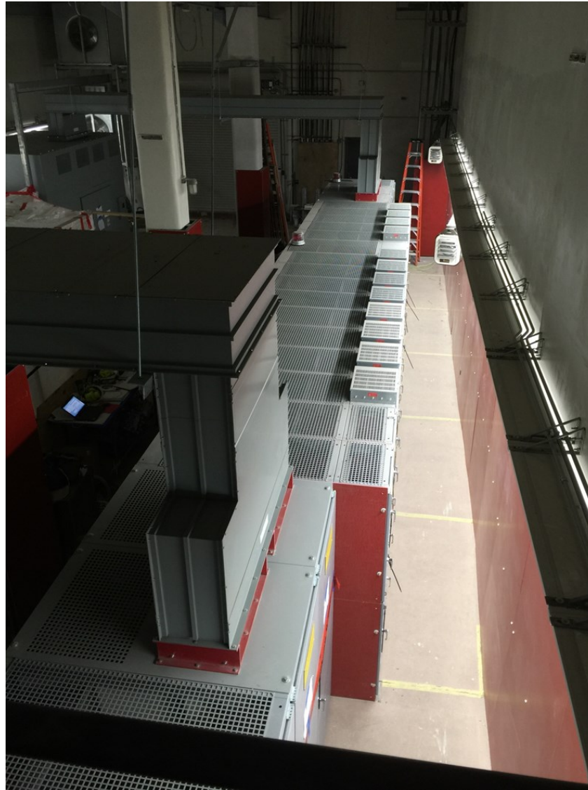
State Substation: New Traction Power Equipment Installed
